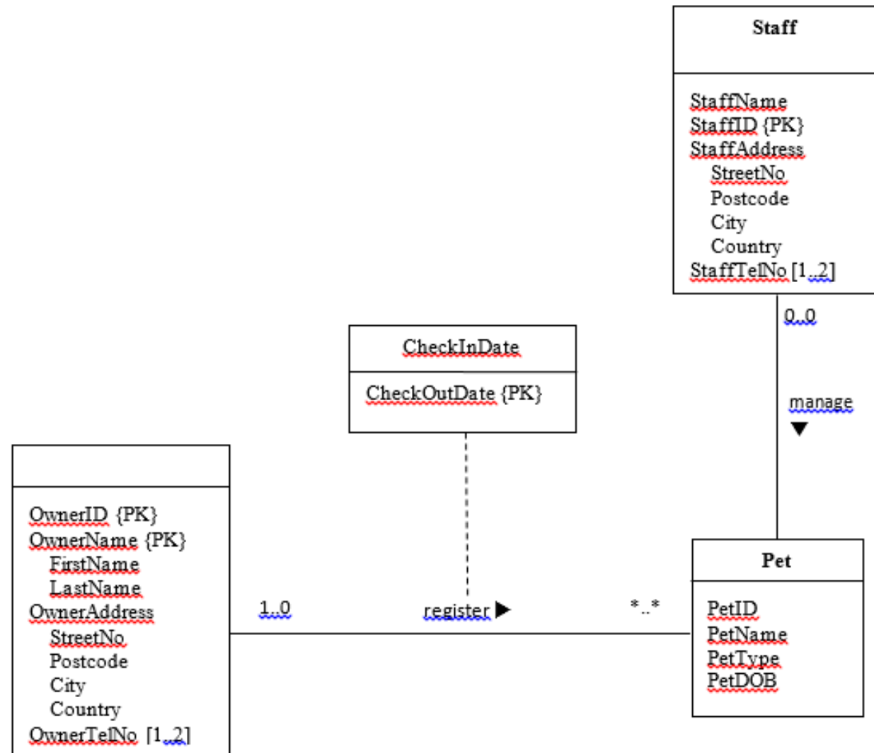
Figure 1: ERD for PET CARE CENTER
