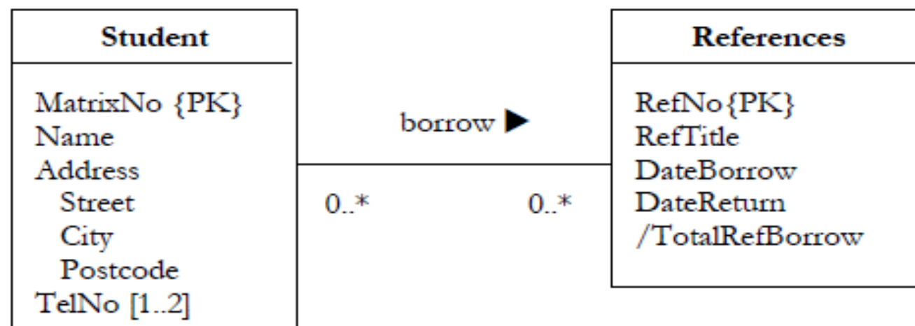
Figure 5: Conceptual Entity Relationship Diagram
